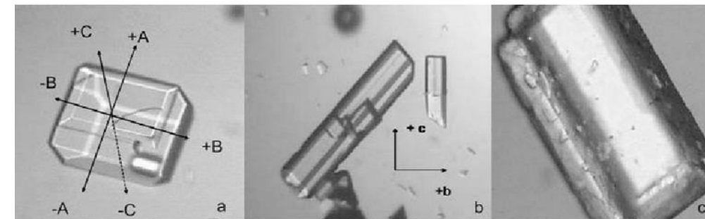
Fig. 14: Effect of dextran on the morphology of sucrose crystals, a) Normal crystal, b) Crystal grown in presence of dextran (needle crystal) and c) Impure particles on crystal surface (crystal grown in technical sucrose solution).
